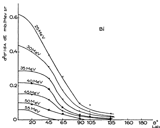
FIG. 6. Differential angular distributions for \alpha particles of several energies for Bi targets.
