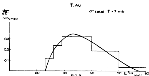
FIG. 8. Integral energy distribution for ^3\text{He} in gold.
